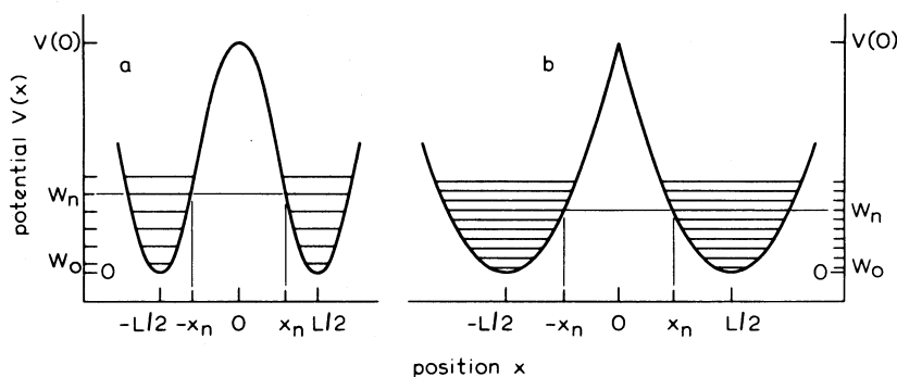
FIG. 3. The parabolic potential barriers considered in the analysis of the low-temperature reorientation frequencies.
