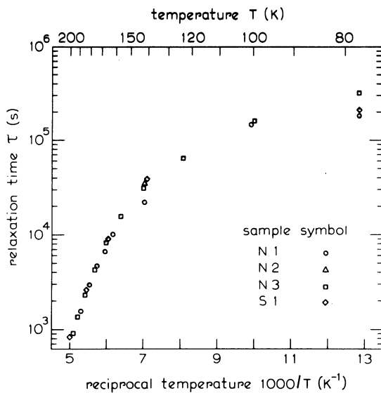
FIG. 1. The reorientation time constant \tau for anneal of stress-induced ordering of substitutional nitrogen in diamond as a function of anneal temperature, as obtained from the static experiments in the low-temperature region.
